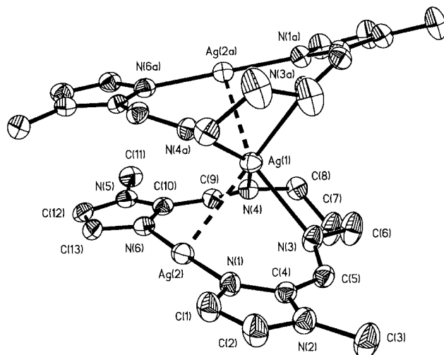
Fig. 4 An ORTEP view of the trinuclear cation in complex 4. Symmetry code: a - x, y, -z + \frac{1}{2} .
